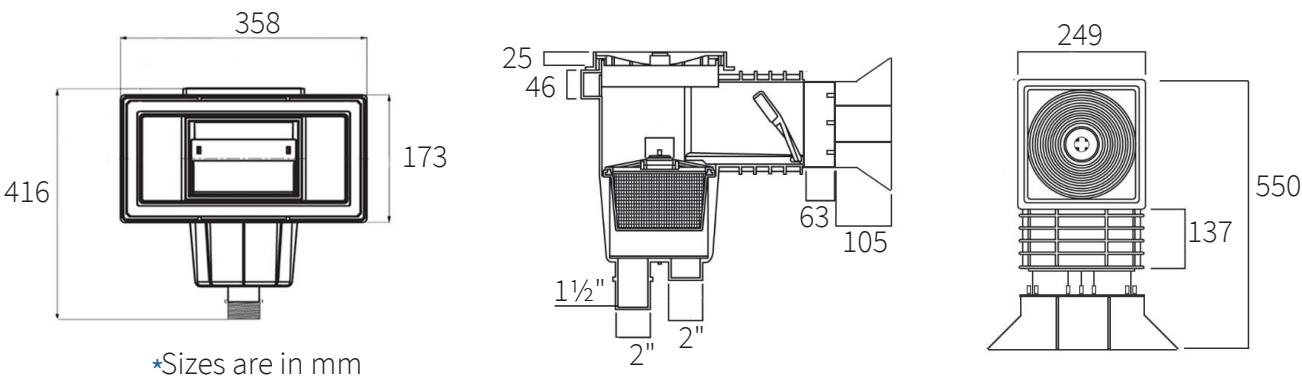
PF-004 Wide Mouth Skimmer with Mouth Extension
